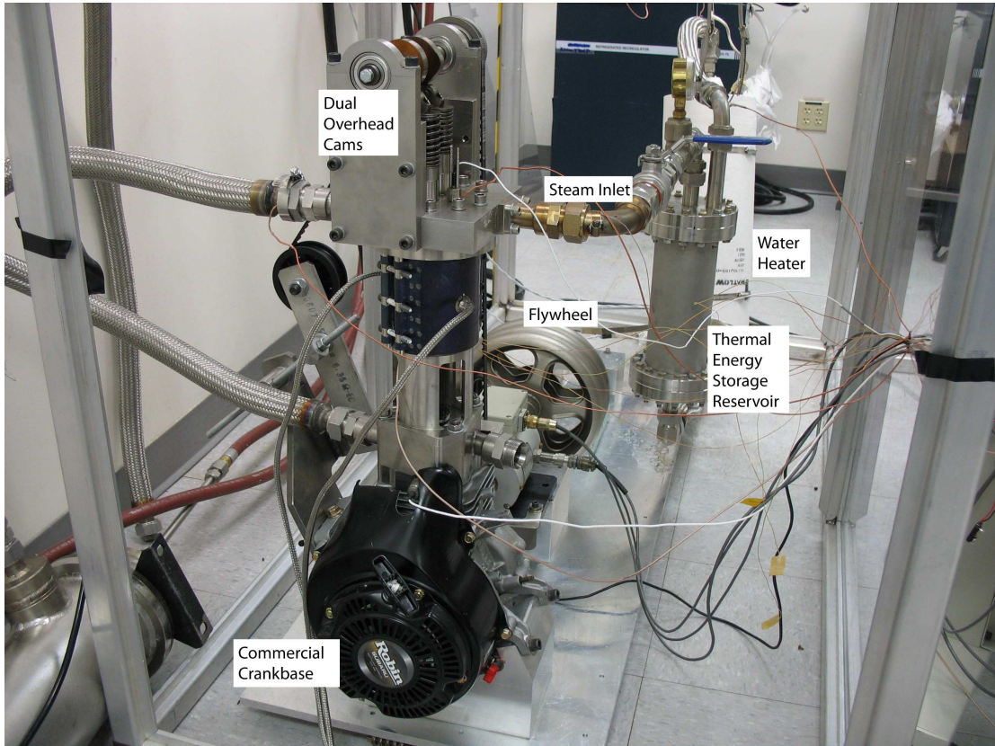
The Gyrosolé™ Heat Powered Engine & Thermal Energy Storage System. (DVD can be provided which shows engine in action.)
