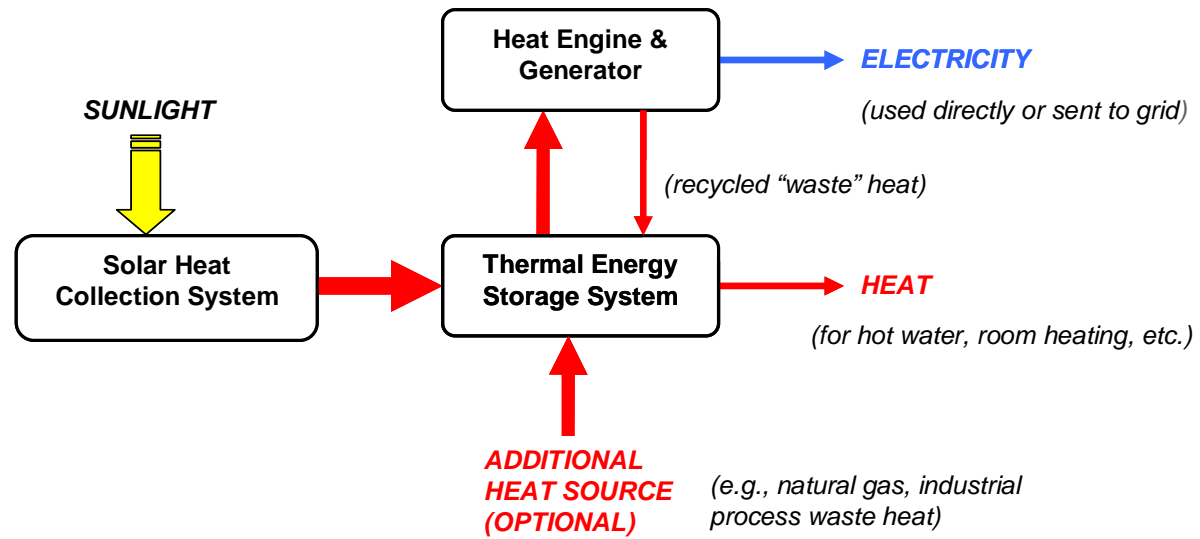
Proposed solar thermal power system schematic
